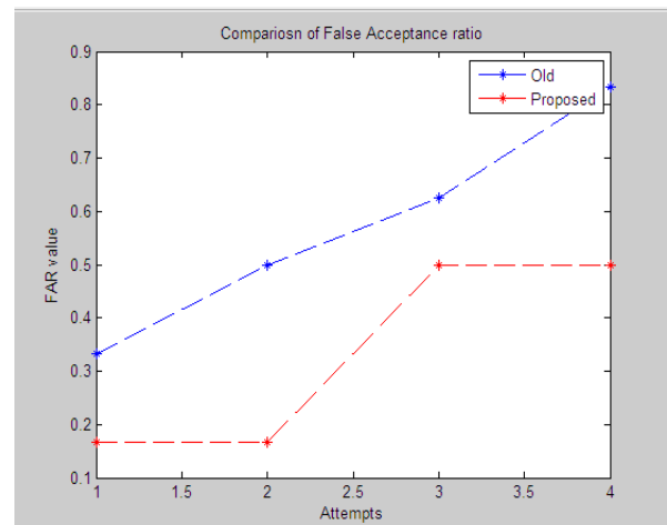
Figure 10 Graph shows the False Acceptance Ratio comparison of proposed and traditional technique.
