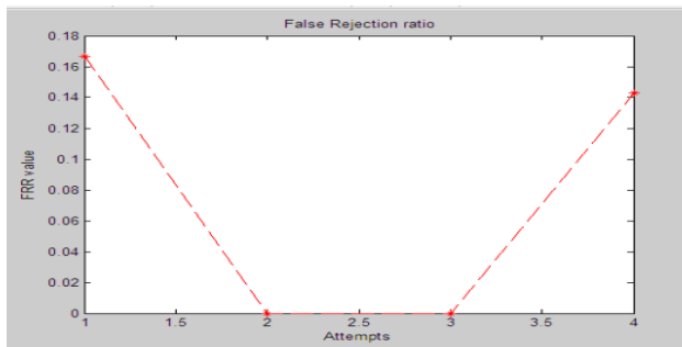
Figure 7 Graph shows the False Rejection Ratio of proposed Work.
