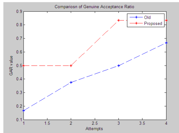
Figure 9 Graph shows the genuine Acceptance Ratio comparison of proposed and traditional technique.
