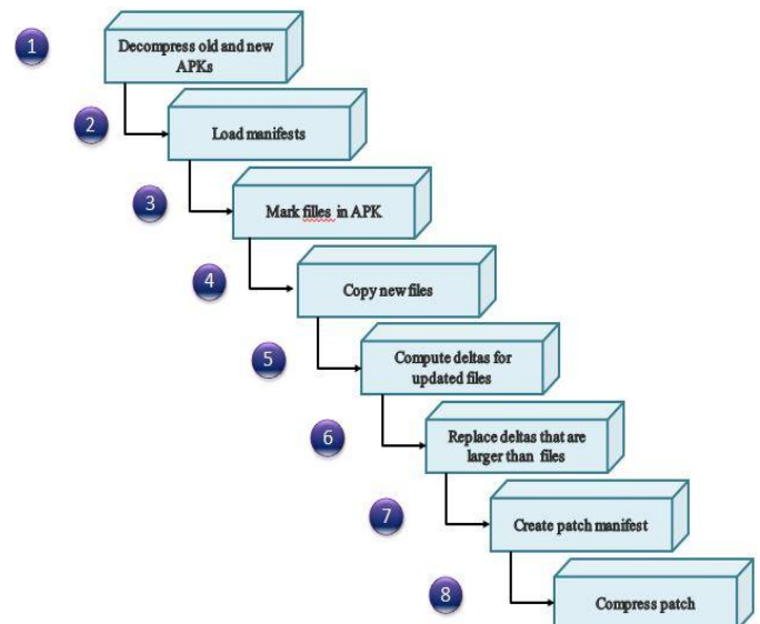
Fig 1. Steps in App Size Reducer patch construction.
