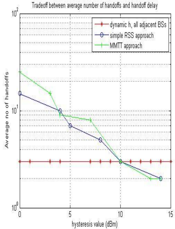
Fig-5: Dynamic hysteresis for handover process
