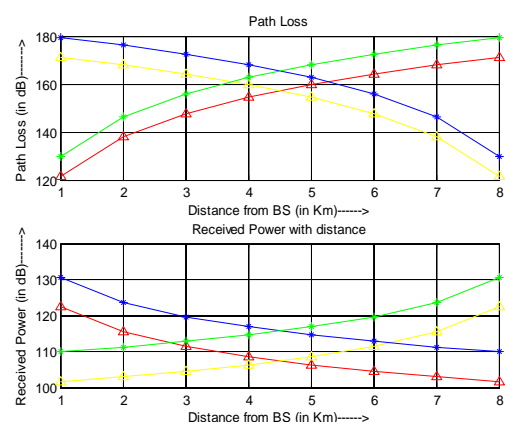
Fig-3: Response of path loss and received signal power
